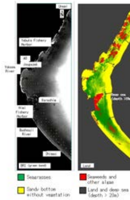
Figure 5 Seagrass distributions detected by the supervised classification with Blue and Green bands of GeoEye-1 taken on November 22, 2014 corrected with the radiometric correction method of the BRI band. The BRI corrected green band (left) and classification results of bottom substrates (right).
