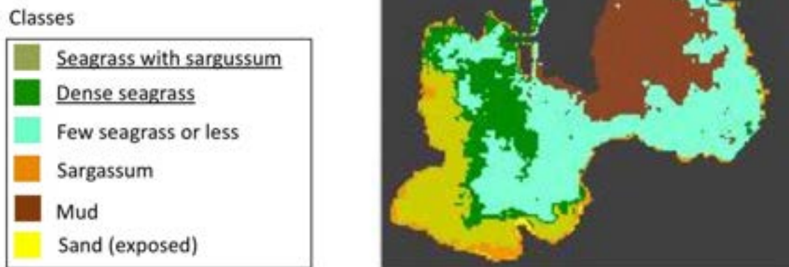
Figure 7 Results obtained by the supervised classification of band ratios of Green/Blue, Green/Red, Blue/Red and Green/Coastal corrected with a radiometric correction method of the Depth Invariant Index (DII) of Landsat 8 OLI on June 1, 2015.
