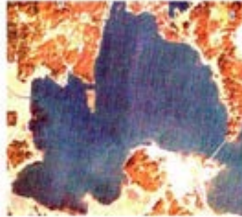
Nov 22, 1991 Unsupervised Classification
