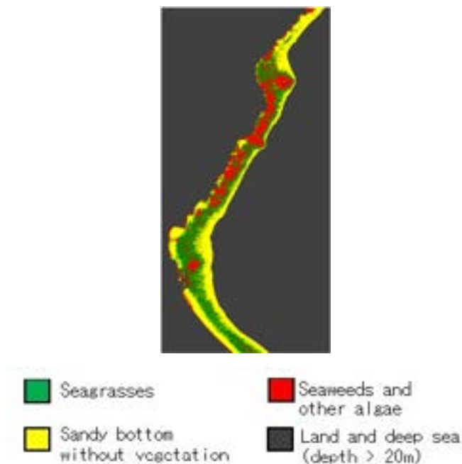
Figure 6 Seagrass distributions detected by the supervised classification of Blue and Green bands of RapidEye taken on March 17, 2016 corrected with the radiometric correction method of the BRI method.
